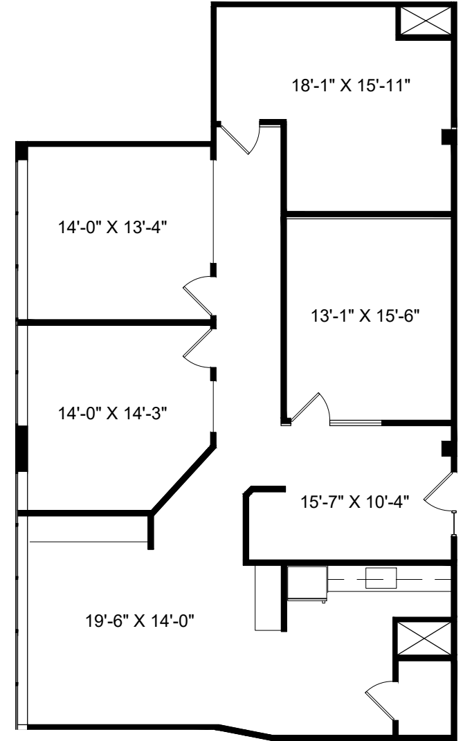
SUITE 209 - 2,049 RSF NOT TO SCALE
